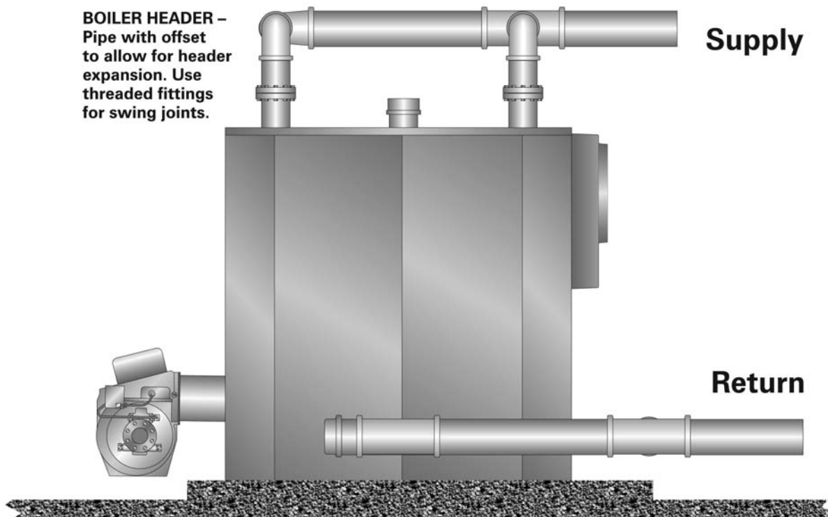
Figure 3.1: Piping Detail, Supply and Return Connections
